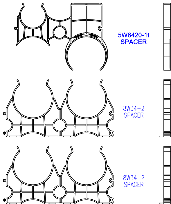
ORTHOGRAPHIC VIEWS OF WUNPEECE SPACERS
