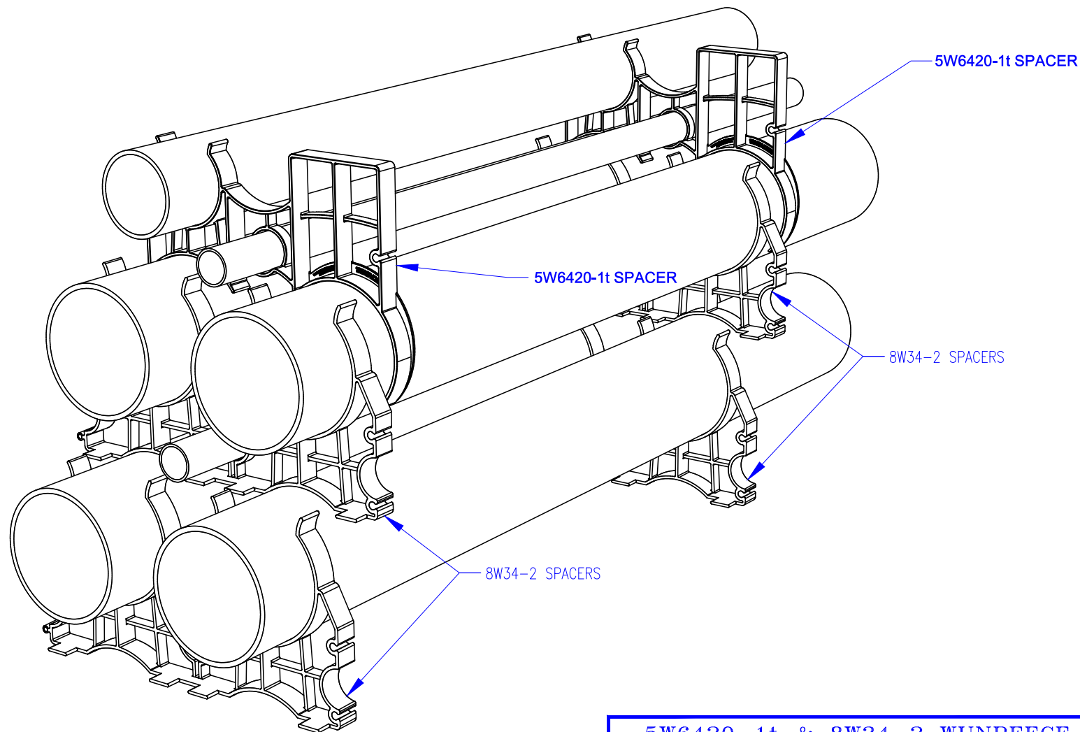
PERSPECTIVE VIEW OF DUCT BANK
