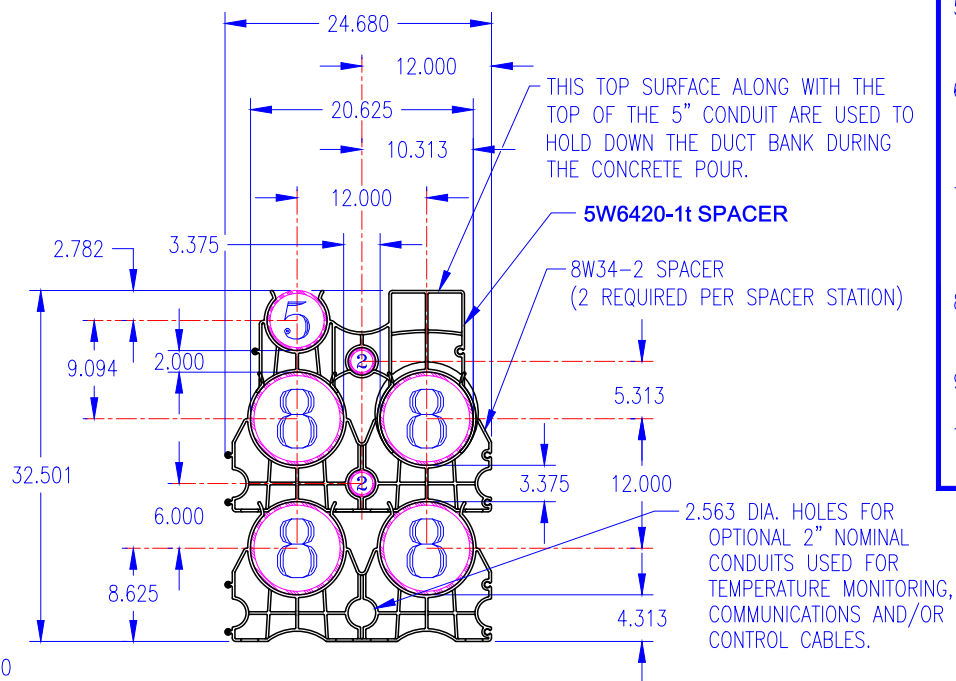
FRONT VIEW OF SPACER STATION
