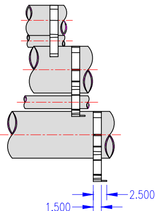
LEFT SIDE VIEW OF SPACER STATION
