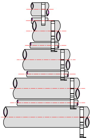
SIDE VIEW OF SPACER STATION
