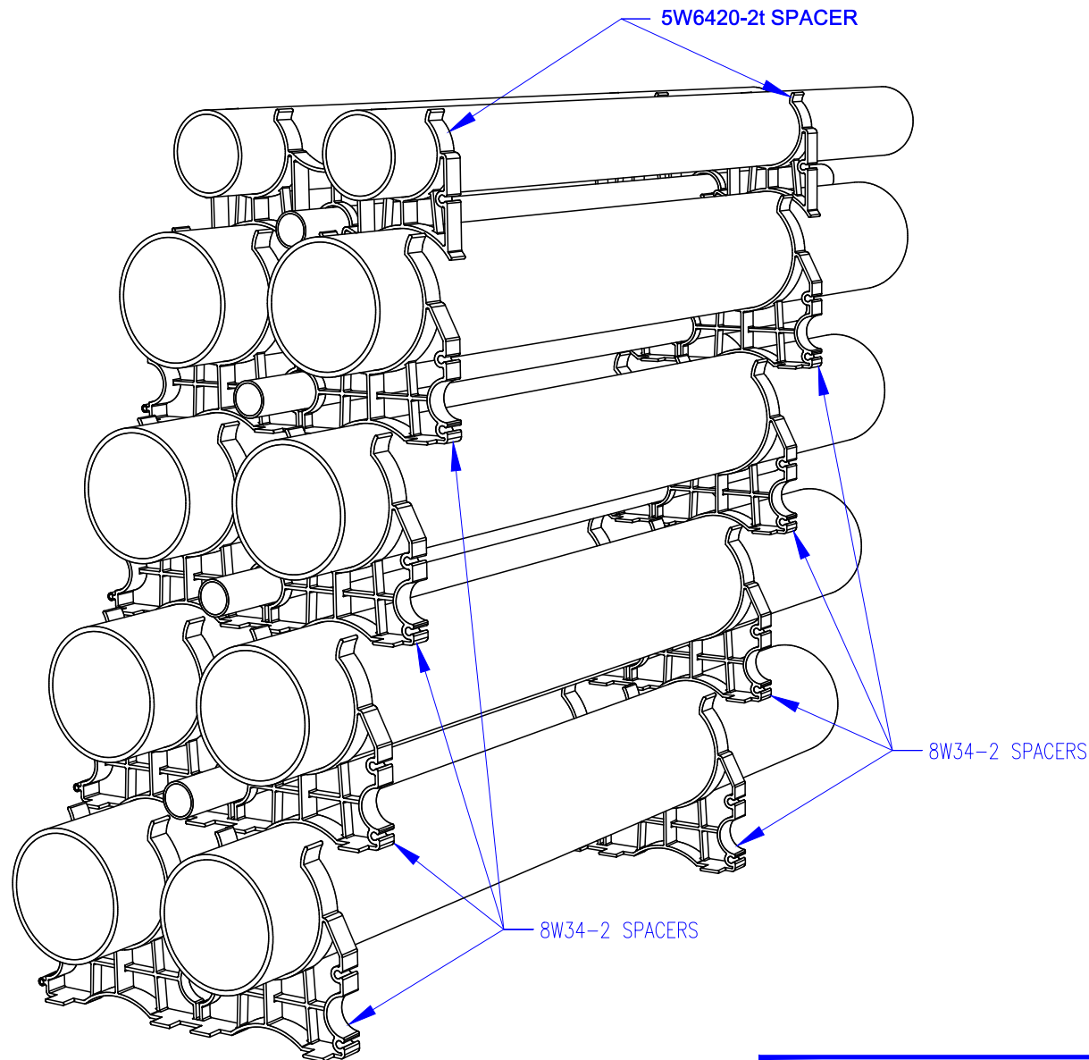
PERSPECTIVE VIEW OF DUCT BANK
