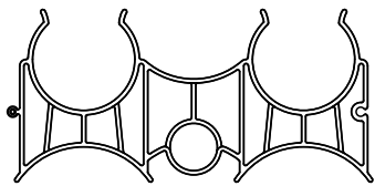
5W6420-2t SPACER
