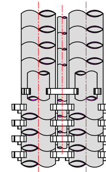
TOP VIEW OF SPACER STATION
