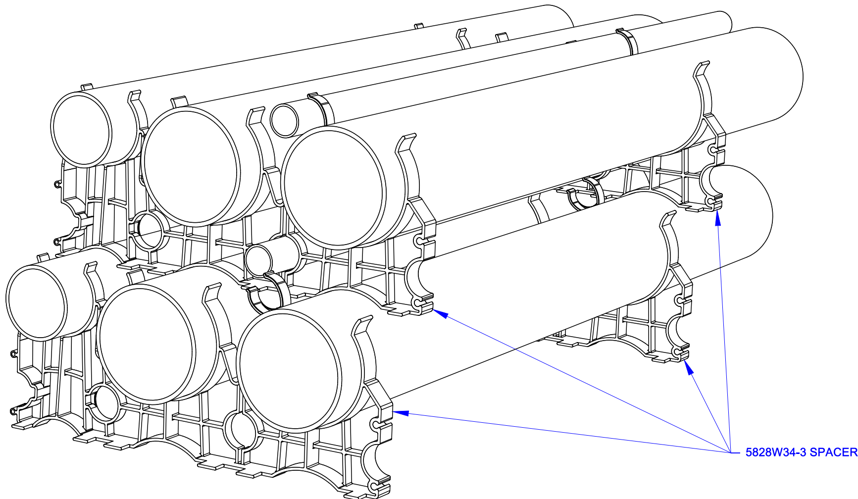
PERSPECTIVE VIEW OF DUCT BANK
