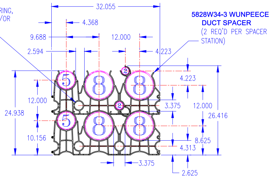
FRONT VIEW OF SPACER STATION
