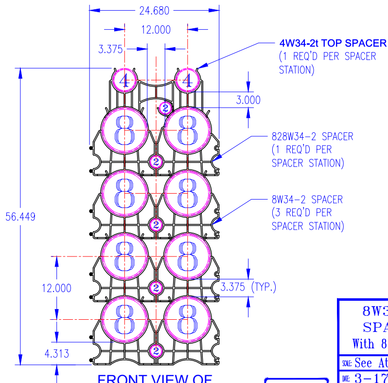
FRONT VIEW OF SPACER STATION
