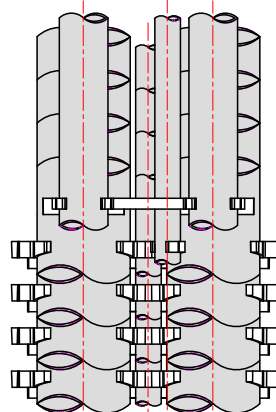
TOP VIEW OF SPACER STATION
