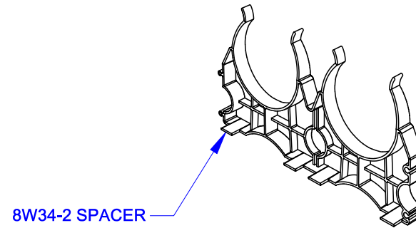
PERSPECTIVE VIEWS OF WUNPEECE SPACERS
