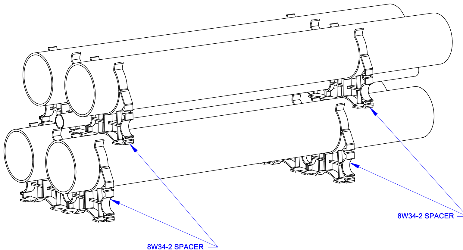
PERSPECTIVE VIEW OF DUCT BANK
