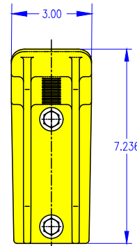
RIGHT END VIEW OF UPPER ARM ONLY
